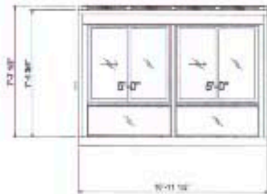
Front Elevation
